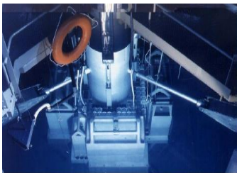
MINERVE Research Reactor for core physic studies
